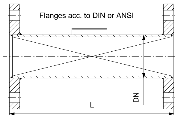
Fig. 2: Fluitec standard mixer CSE-B
